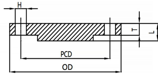
Large Bore Blind Flanges ASME B16.47A
